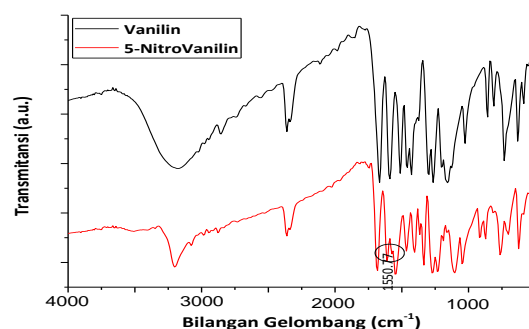
Figure 4. FTIR spectra of 5-nitrovanillin compound
