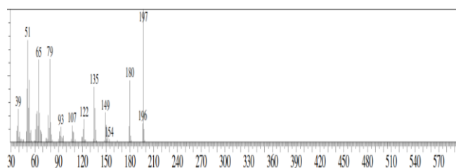
Figure 5. Mass spectrum of the compound 5-nitrovanillin
