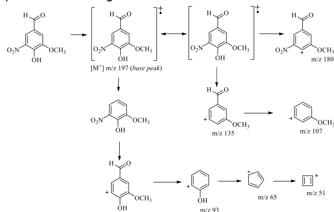
Figure 6. The fragmentation pattern of 5-nitrovanillin compound
