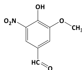
Figure 2. 5-nitrovanillin compound structure
