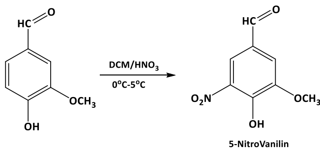
Figure 3. 5-nitrovanillin synthesis pathway
