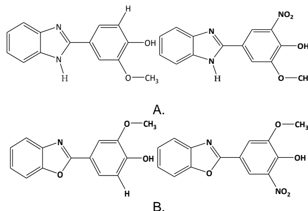
Figure 1. Comparison of the sensor structure: A) S1 with S2; B) S3 with S4.
