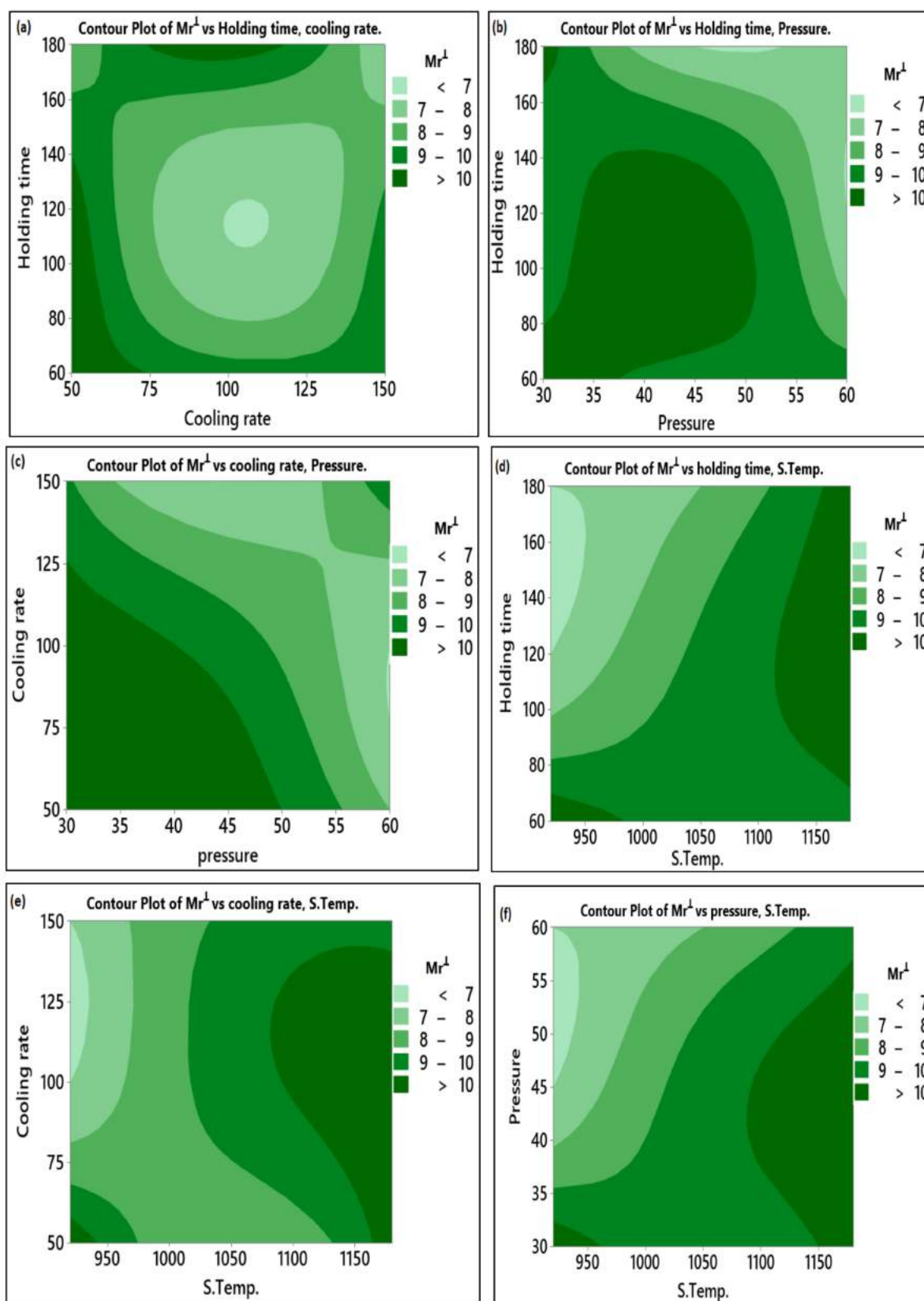
Figure 11. Contour plot for Mr^I : (a) Holding time vs. cooling rate; (b) Holding time vs. pressure; (c) Cooling rate vs. pressure; (d) Holding time vs. S. temp.; (e) Cooling rate vs. S. temp.; (f) Pressure vs. S. temp.
